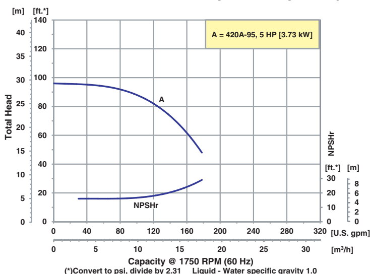
Performance of 2" x 1-1/2" Straight Centrifugal Pump
