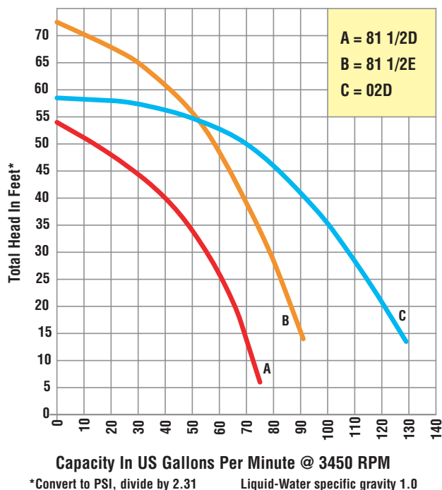
Performance of Self-Priming Pedestal Pumps
